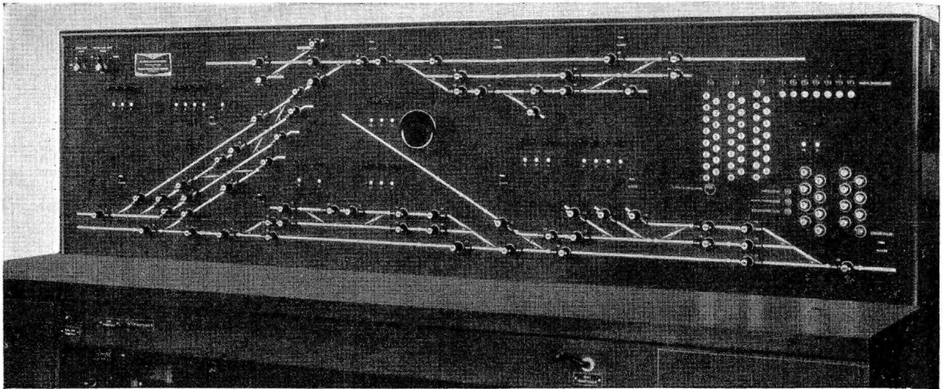
The control panel of the interlocking on Oakland mole
