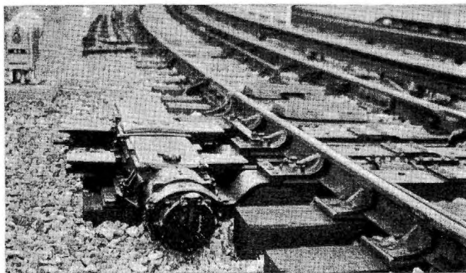
The ties are dapped so the rods can be straight. The plates extend under machine
