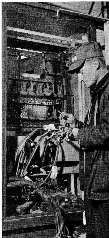
Left—Interior of outdoor instrument case showing Type-B relays and code transmitter Below—Rear of case showing method used when connecting the incoming cable wires
