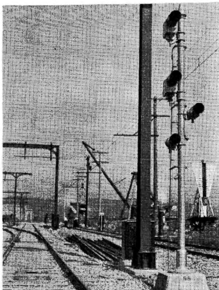
Eastward signal 98 at Oakland showing operative units and markers
