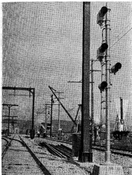
Interlocking signal 98 at Oakland showing operative units and markers
