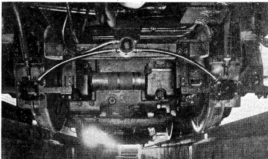
The receiver coils are mounted ahead of the leading wheels of a car and about six inches above the level of the top of the rail
