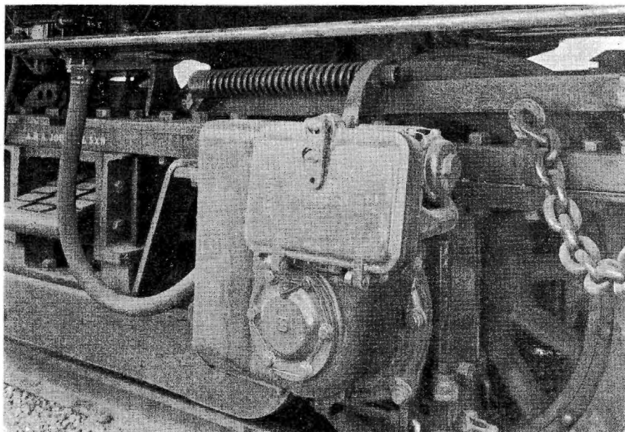
The speed governor is mounted on the end of the car truck being geared to the end of the axle to drive a governor which actuates contacts
