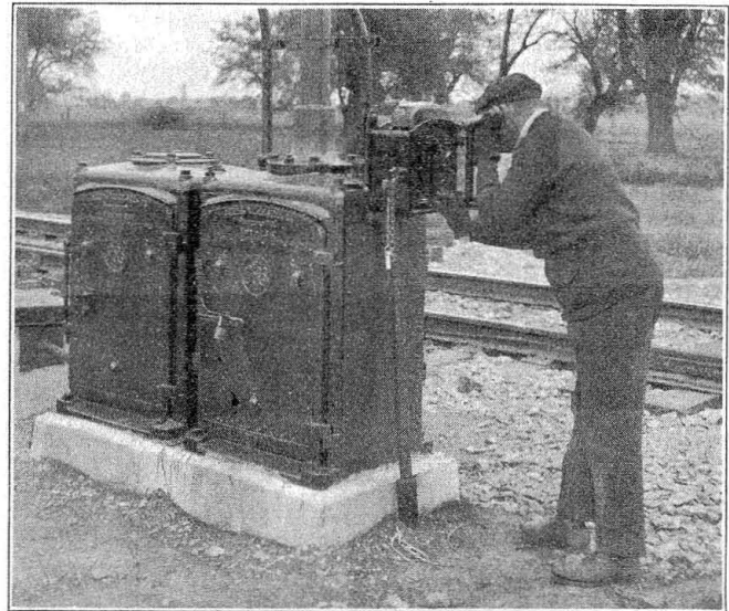
Fig. 4—Trainman calling dispatcher by roadside telephone
