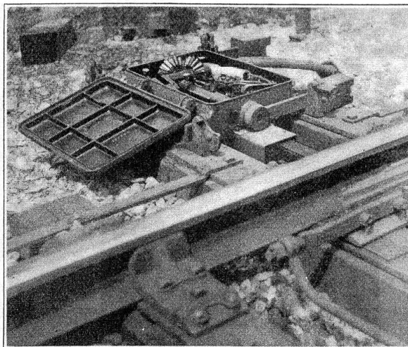
Fig. 20—Dual control selector
