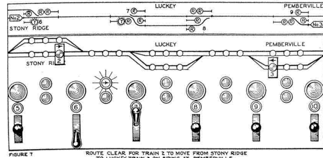
FIGURE 7 ROUTE CLEAR FOR TRAIN 2 TO MOVE FROM STONY RIDGE TO LUCKEY, TRAIN 3 ON SIDING AT PEMBERVILLE.
