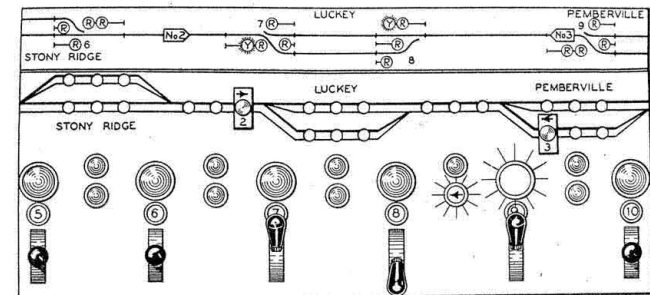
FIGURE 9 TRAIN 2 HAS NOT ARRIVED AT LUCKEY AND TRAIN 3 IS LEAVING PEMBERVILLE.
